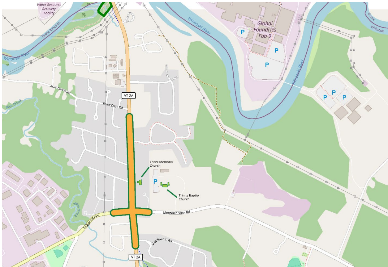
Crews widen the roadway and install drainage along VT 2A southbound between Meadowrun Road and Industrial Avenue in Williston, VT.
