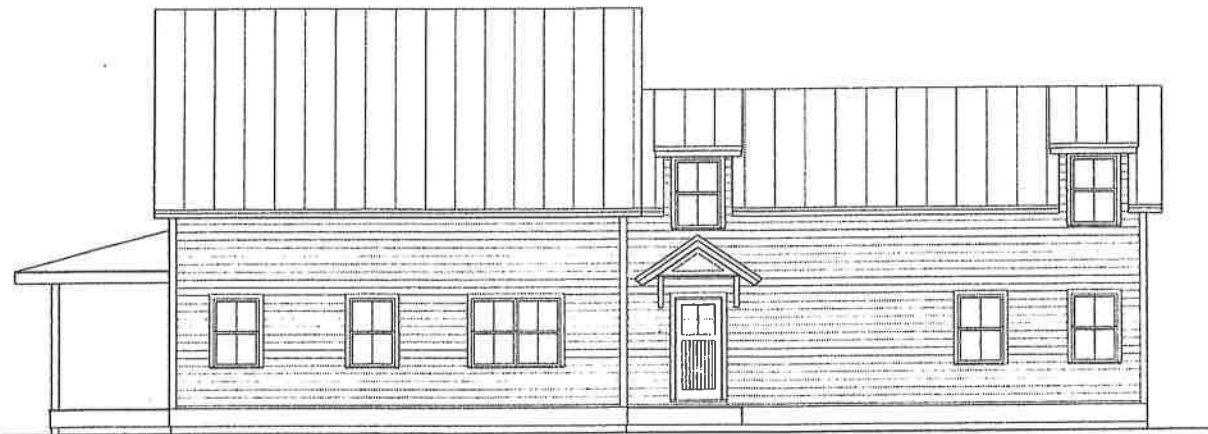
WEST ELEVATION
