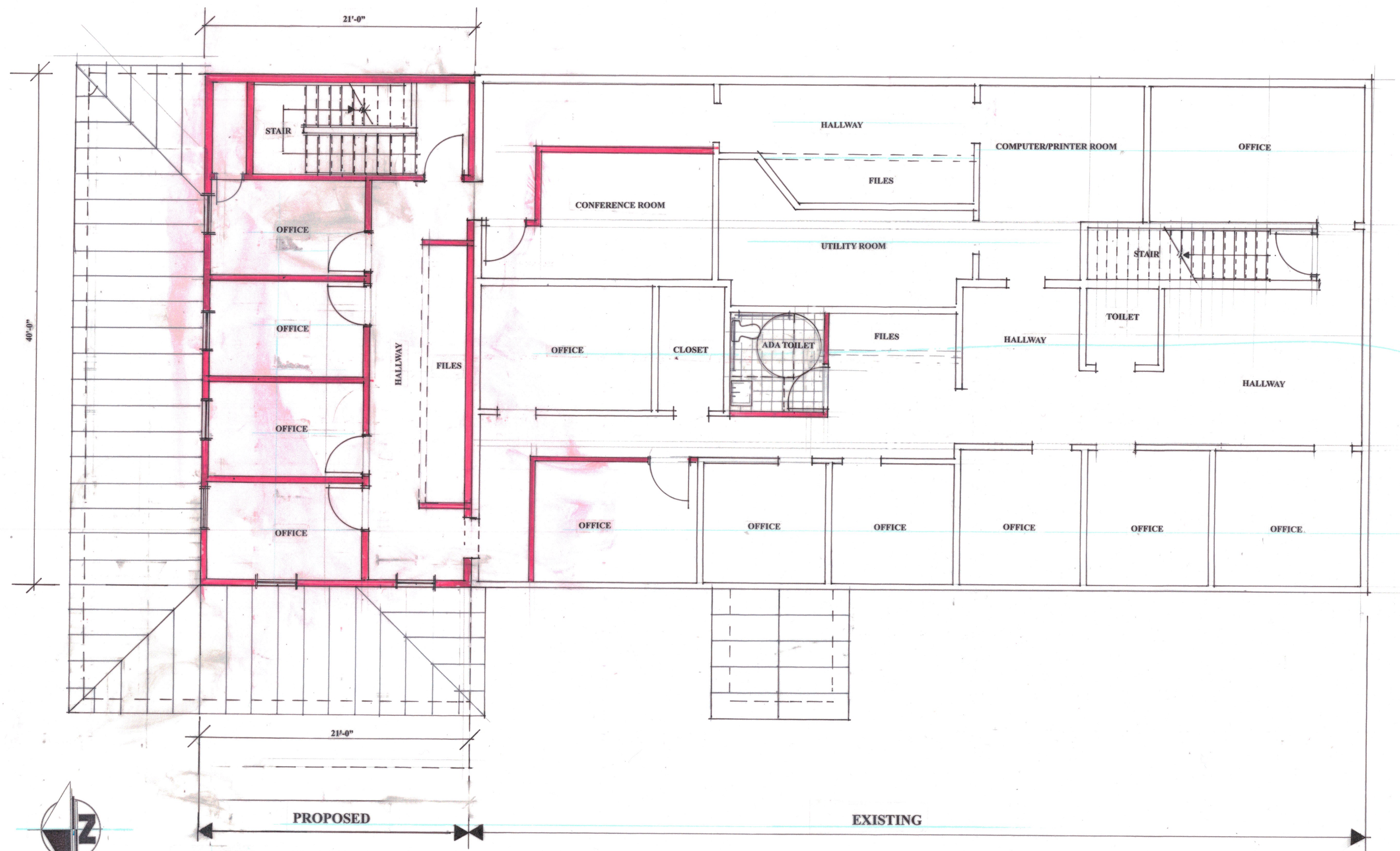
SECOND FLOOR PLAN 1/4" = 1'-0"
