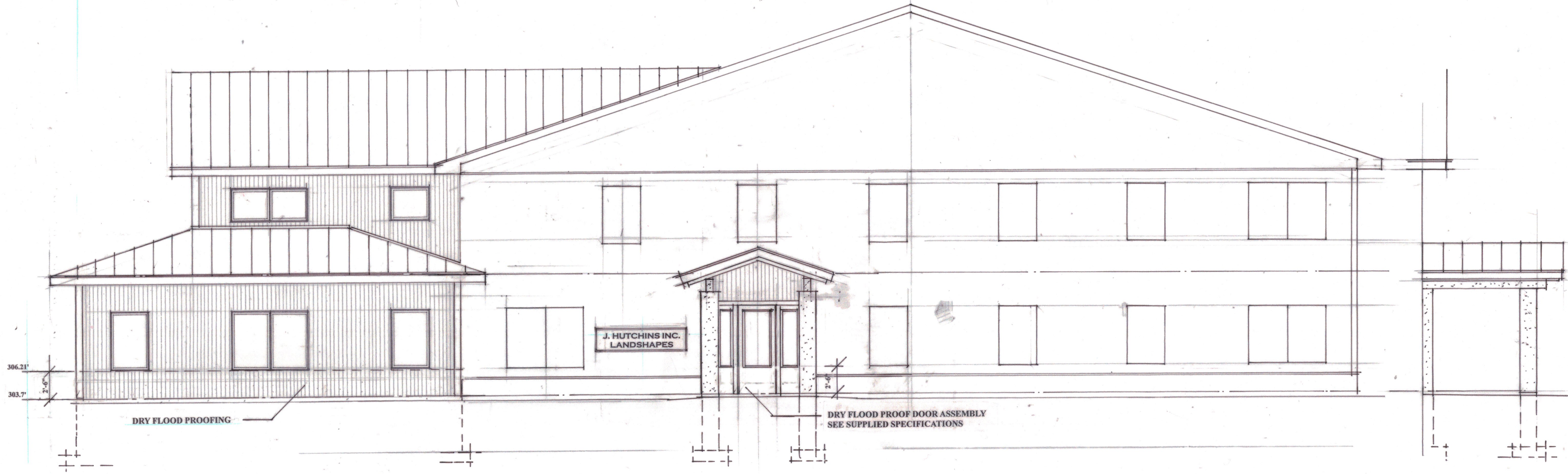
WEST ELEVATION 1/4" = 1' - 0"
