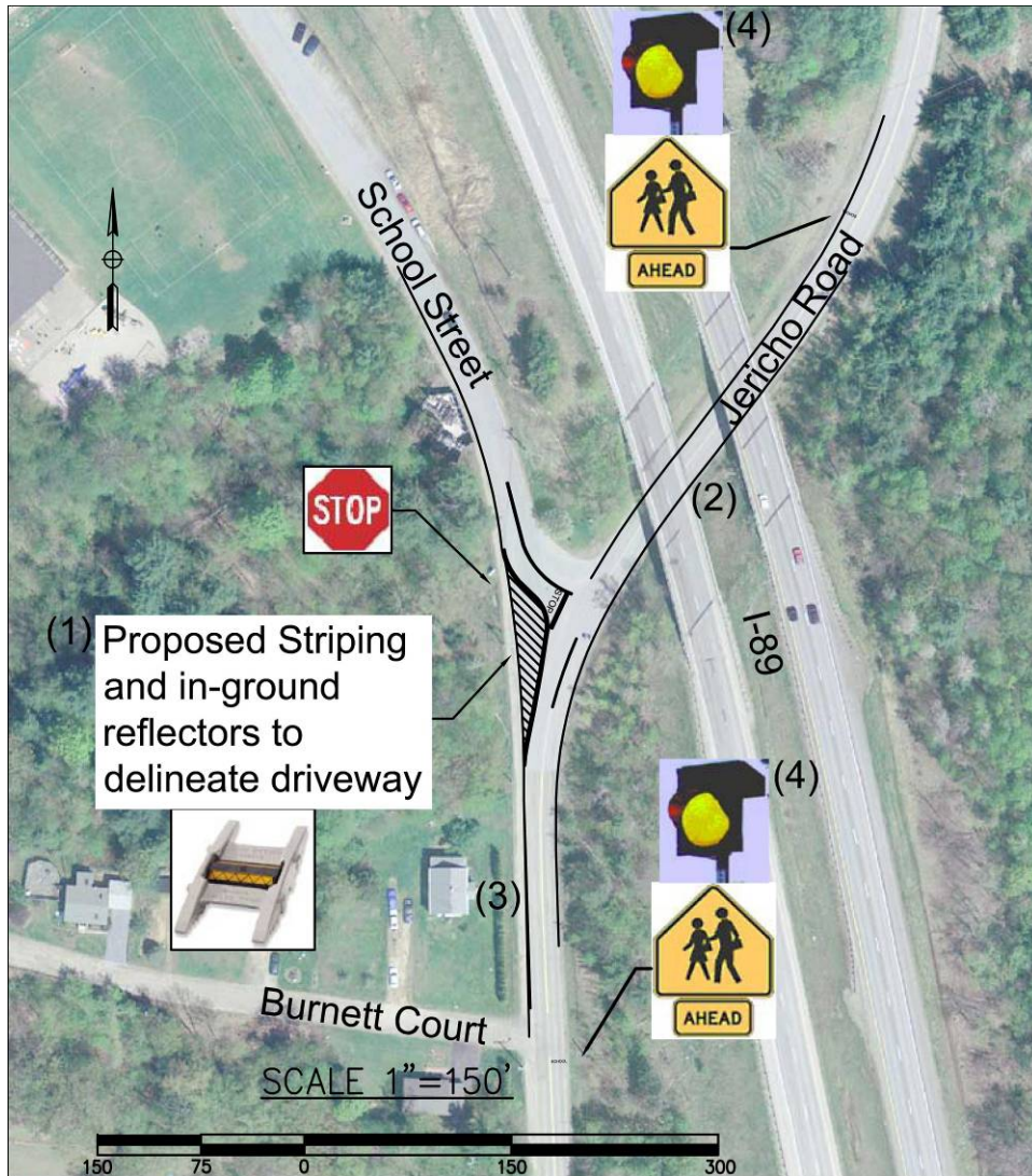
Figure 1: Design Schematic
